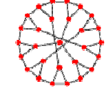
28-cubic graph J
