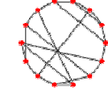
14-cubic graph 257
