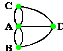
The Seven Bridges of Königsberg
