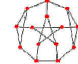
14-cubic graph 388
