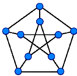
Single Star Snark (Petersen Graph)
