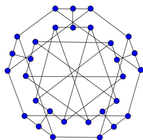
Double Star Snark
