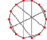
14-cubic graph 372
