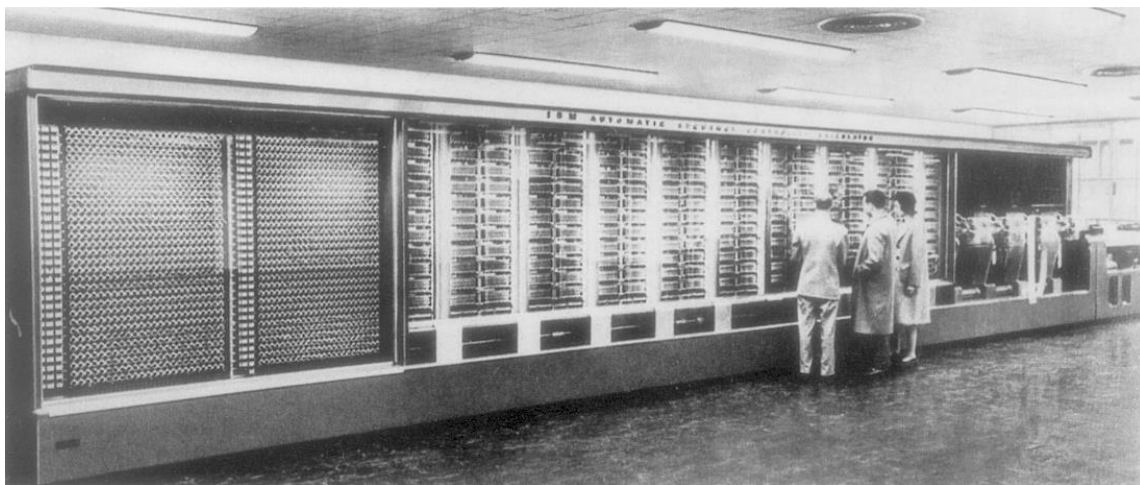
Harvard Mark I , The first large scale, automatic, general purpose, electromechanical calculator (1944)
